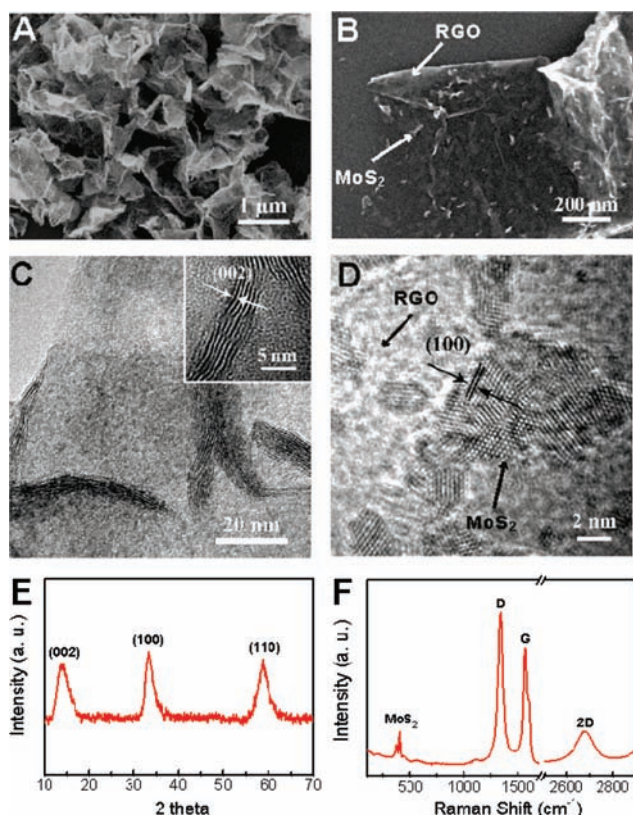
Figure 2. \text{MoS}_2 nanoparticles on graphene in the \text{MoS}_2/\text{RGO} hybrid. (A, B) SEM images of the \text{MoS}_2/\text{RGO} hybrid. (C) TEM image showing folded edges of \text{MoS}_2 particles on RGO in the hybrid. The inset shows a magnified image of the folded edge of a \text{MoS}_2 nanoparticle. (D) High-resolution TEM image showing nanosized \text{MoS}_2 with highly exposed edges stacked on a RGO sheet. (E) XRD pattern and (F) Raman spectrum of the hybrid.
