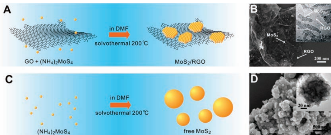
Figure 1. Synthesis of \text{MoS}_2 in solution with and without graphene sheets. (A) Schematic solvothermal synthesis with GO sheets to afford the \text{MoS}_2/\text{RGO} hybrid. (B) SEM and (inset) TEM images of the \text{MoS}_2/\text{RGO} hybrid. (C) Schematic solvothermal synthesis without any GO sheets, resulting in large, free \text{MoS}_2 particles. (D) SEM and (inset) TEM images of the free particles.
